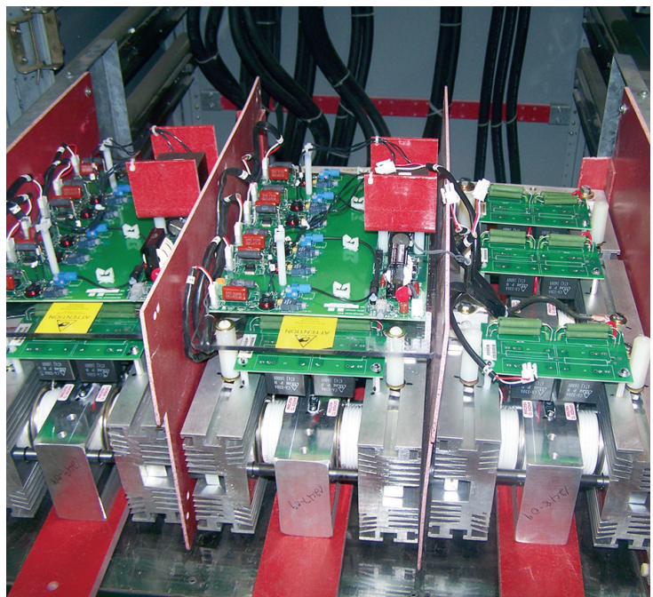
Medium Voltage Control Section
