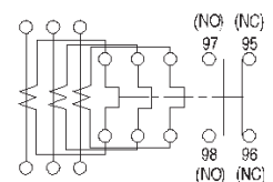
Wiring Diagram
