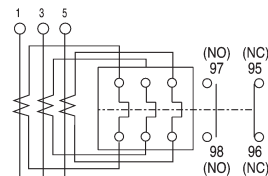
Wiring Diagram
