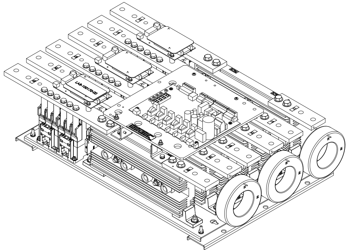
FULL ASSEMBLY
