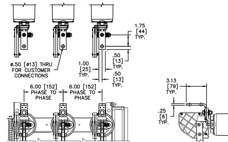
MATERIAL: .25" THICK TIN PLATED COPPER
