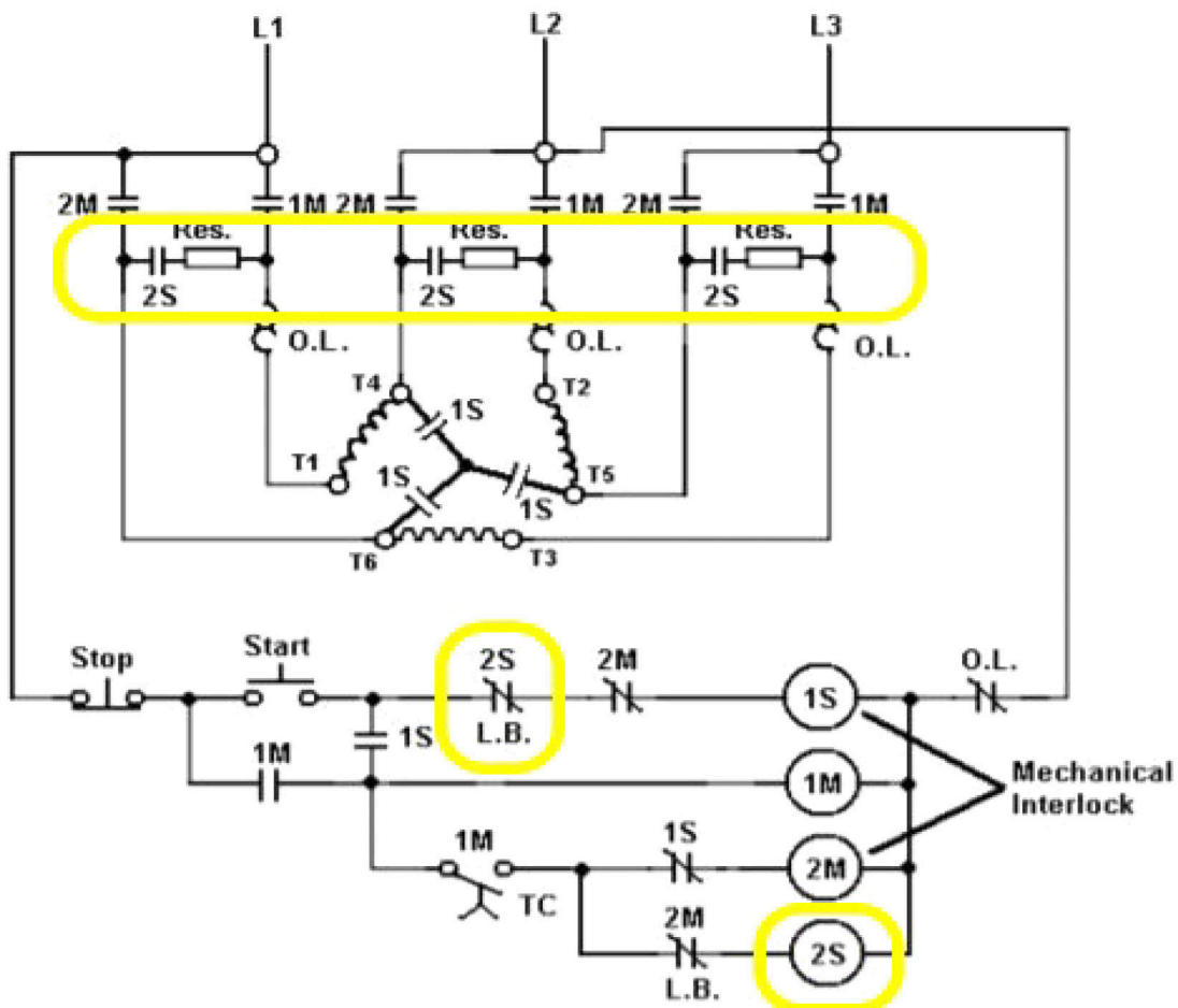
Figure 4. Typical – Closed transition type Wye-Delta starter. Added components: 2 S contactor, resistors.
