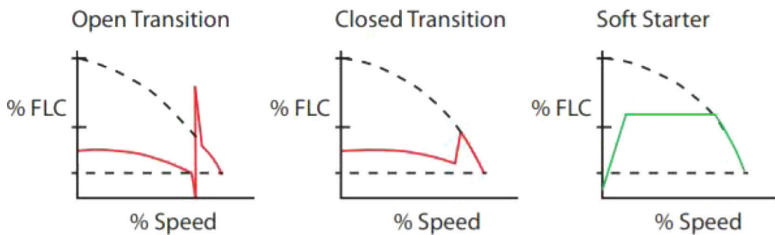
Figure 6. A graphical representation of the current and speed relationships between the various methods.
