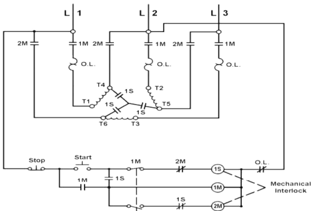
Figure 3. Typical – Open transition type Wye-Delta starter
