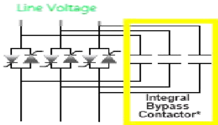
Figure 5. Typical – Basic soft starter configuration
