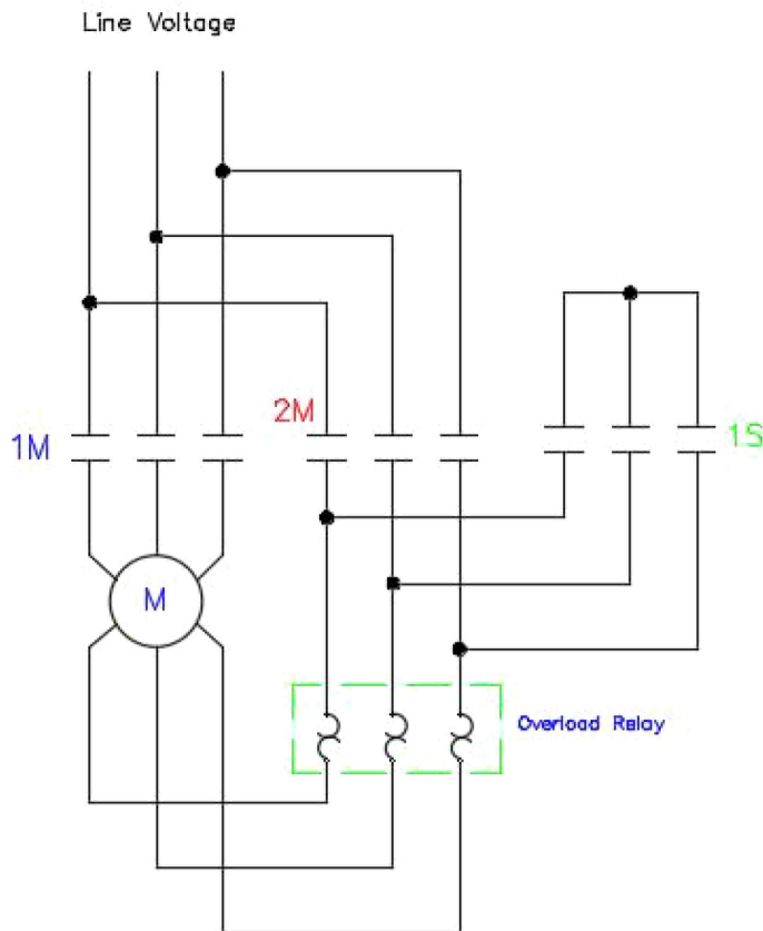
Figure 2. Basic Wye-Delta starter configuration
