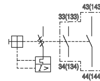
Connection Diagram
