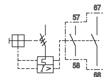
Connection Diagram
