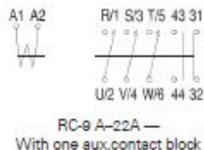
RC-9 A-22A — With one aux.contact block
