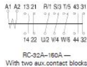
RC-32A-150A — With two aux.contact blocks
